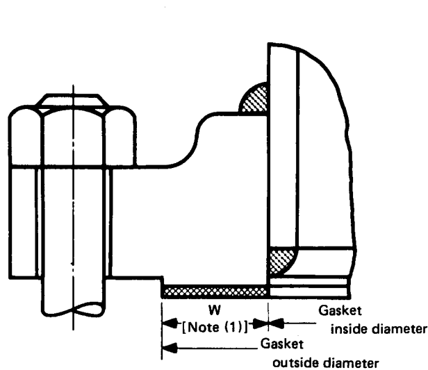
FIG. E2 3 SLIP-ON RAISED FACE WIDTH GASKET
