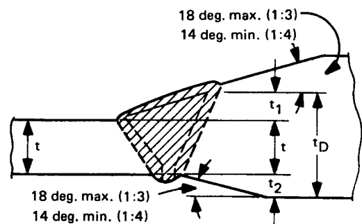
FIG. 14 BEVEL FOR COMBINED THICKNESS 1-4
