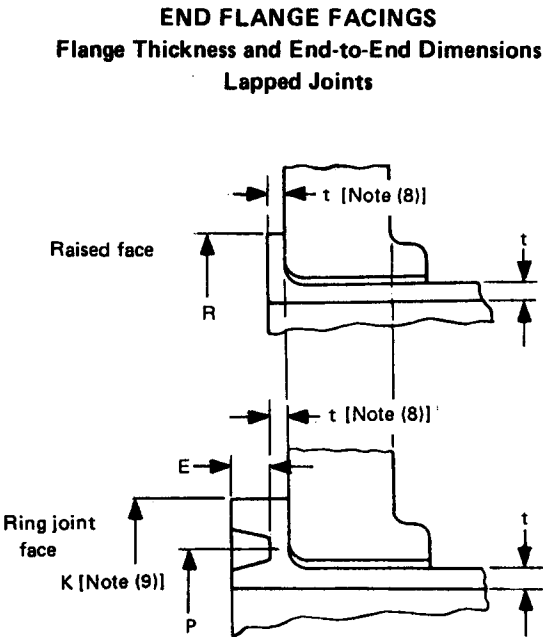
FIG. 7 END FLANGE FACINGS AND THEIR RELATIONSHIP TO FLANGE THICKNESS AND CENTER-TO-END AND END-TO-END DIMENSIONS 1,3 (CONT'D)
