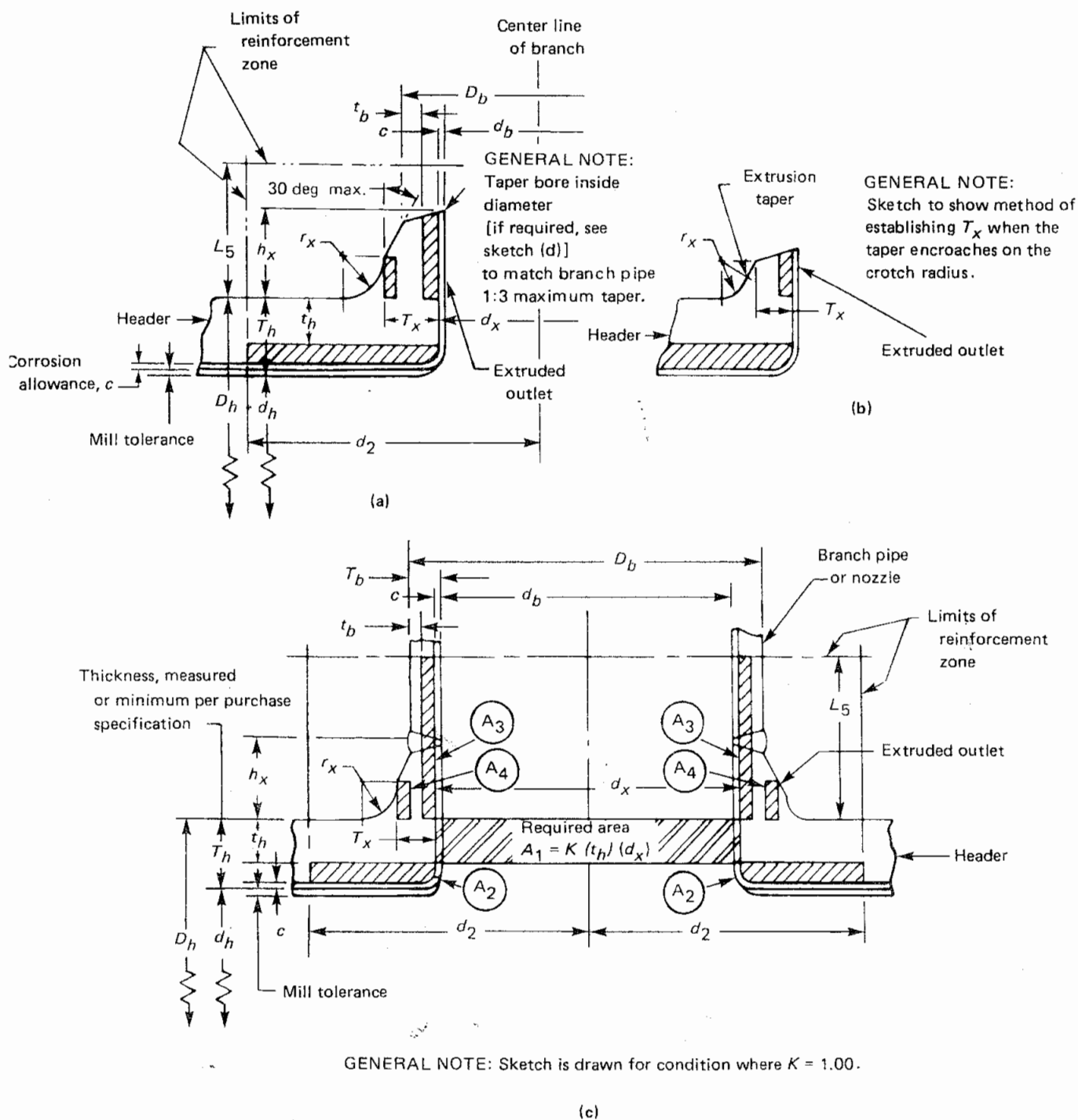
Fig. 304.3.4 Extruded Outlet Header Nomenclature
