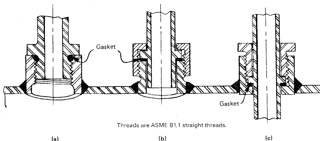
Fig. 335.3.3 Typical Threaded Joints Using Straight Threads
