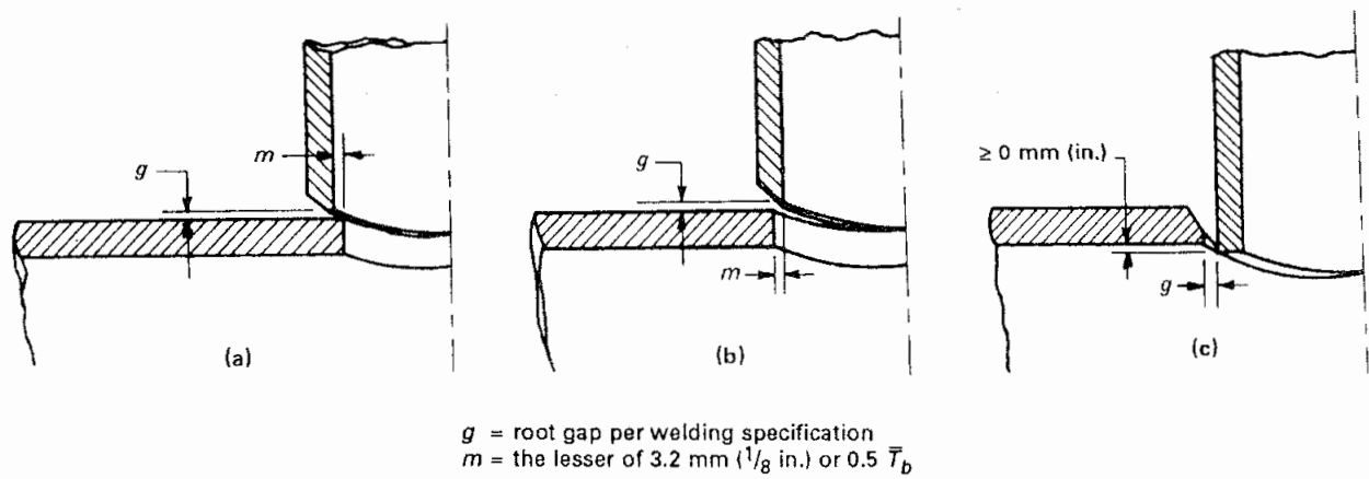
Fig. 328.4.4 Preparation for Branch Connections
