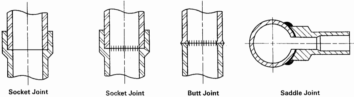
FIG.A328.5.3 THERMOPLASTIC SOLVENT CEMENTED JOINT
