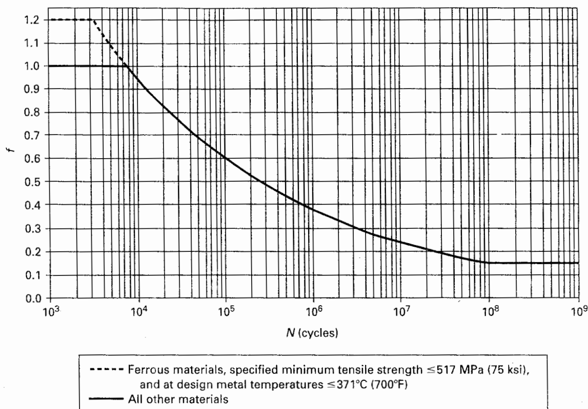
Fig. 302.3.5 Stress Range Reduction Factor, f
