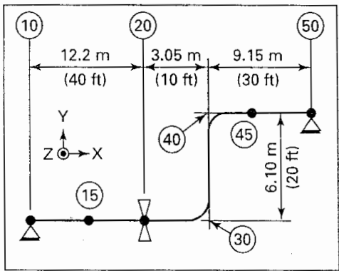
Fig. S301.1 Simple Code Compliant Model
