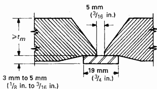
(a) Butt Joint With Bored Pipe Ends and Solid or Split Backing Ring [Note (1)]
