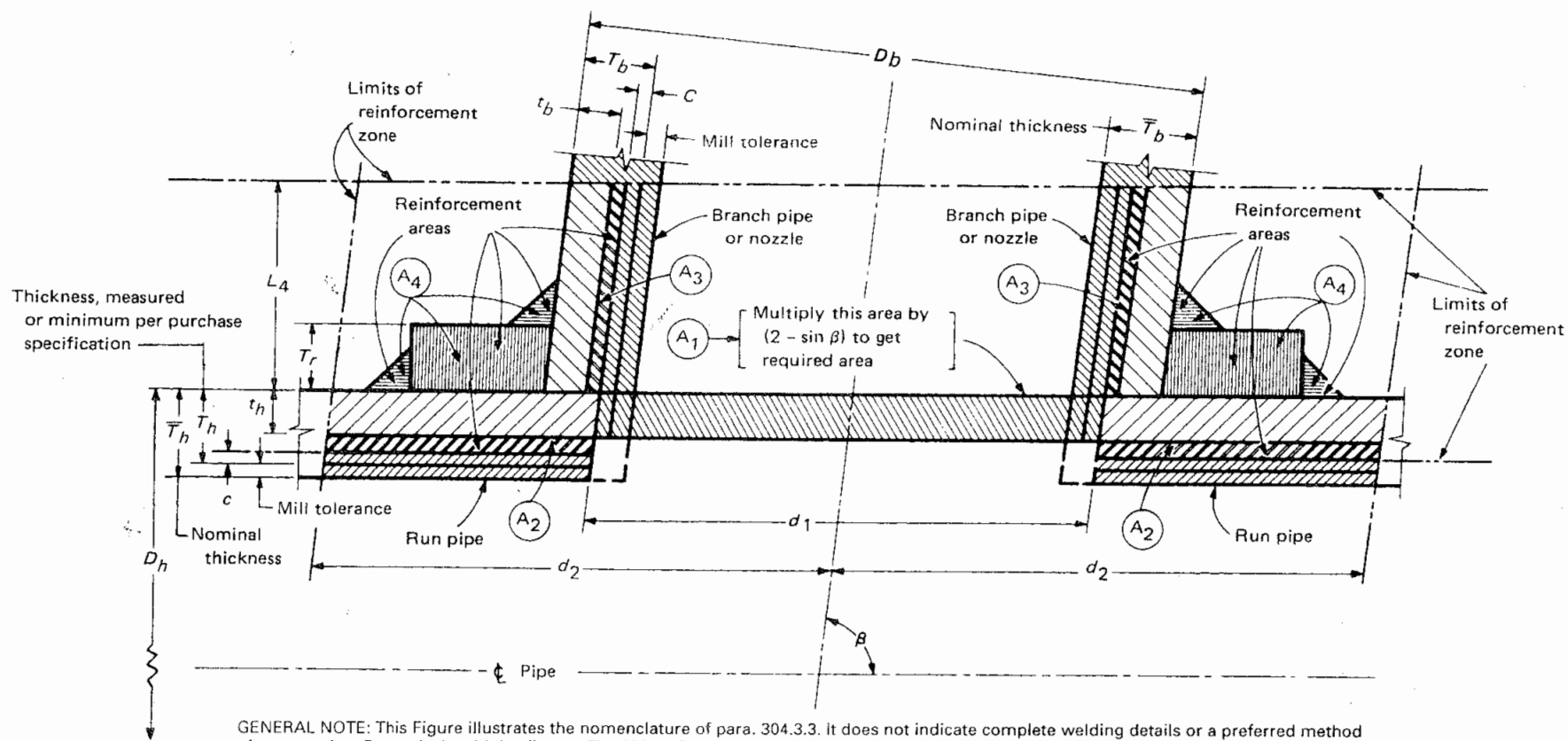
Fig. 304.3.3 Branch Connection Nomenclature
