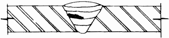
(b) Lack of Fusion Between Adjacent Passes
