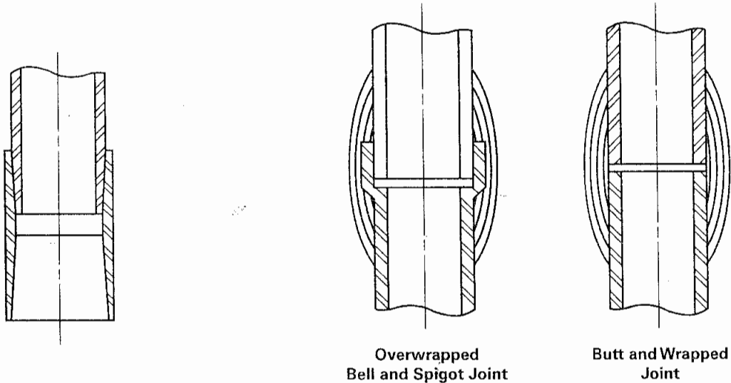
FIG.A328.5.6 FULLY TAPERED THERMOSETTING ADHESIVE JOINT
