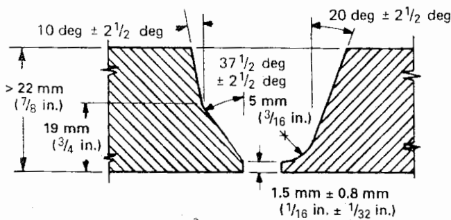
(b) Wall Thickness Over 22 mm ( \frac{7}{8} in.)
