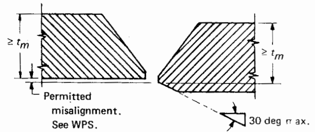
(a) Thicker Pipe Taper-Bored to Align
