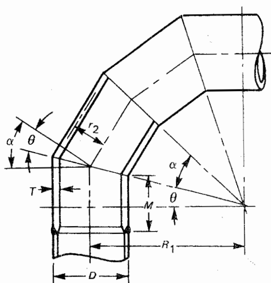
Fig. 304.2.3 Nomenclature for Miter Bends
