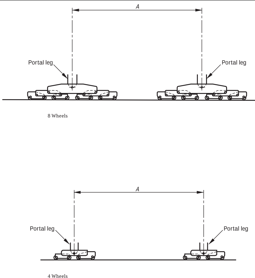
Figure 36 — Container crane bogie with alternative number of wheels
