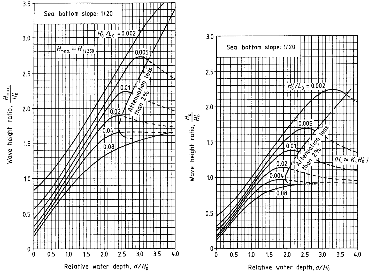
Figure 3d) — Wave shoaling and estimation of wave height in the surf zone (continued)
