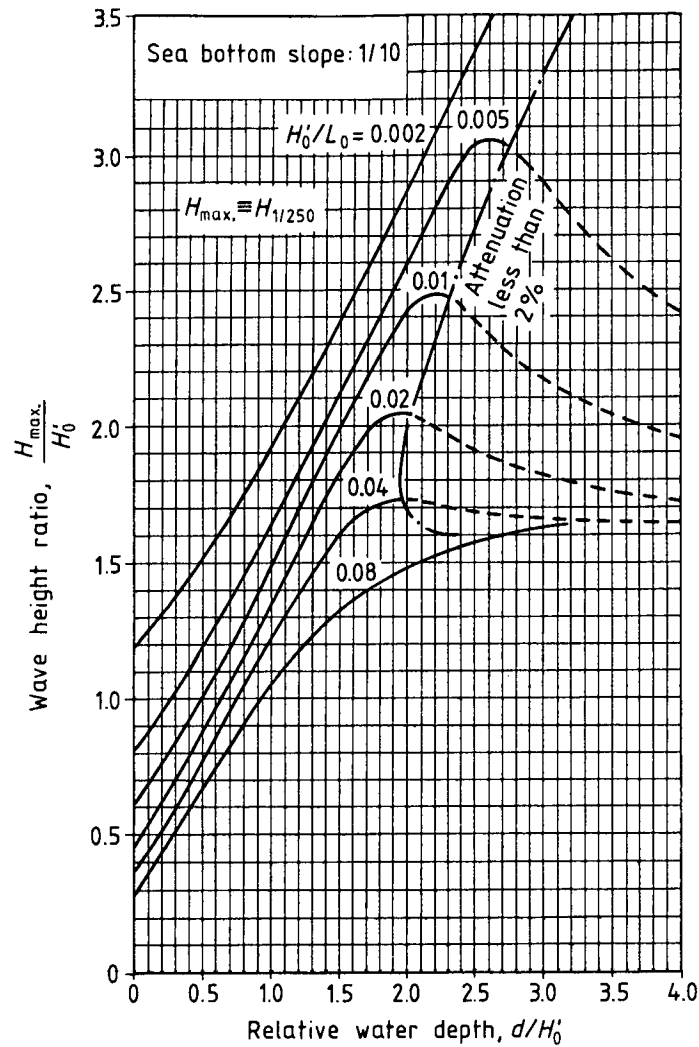
Figure 3c) — Wave shoaling and estimation of wave height in the surf zone (continued)
