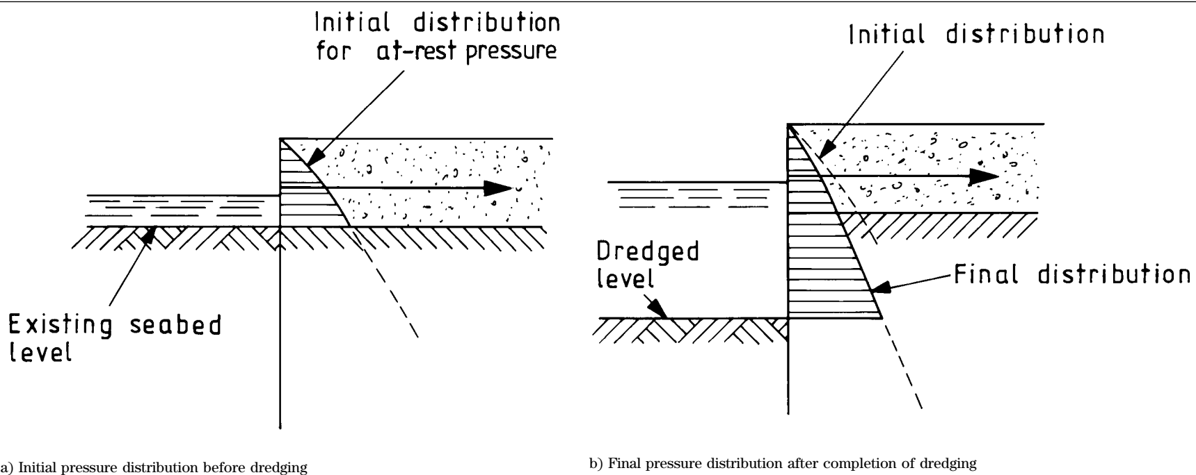
Figure 51 — Active pressure distribution on anchored single-wall structure where filling is placed before dredging
