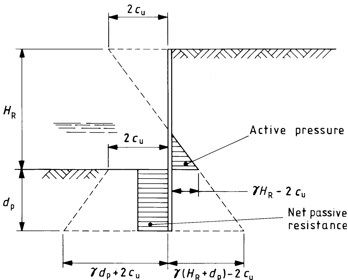
Figure 53 — Distribution of active pressure and passive resistance for total stress conditions in normally- and lightly over-consolidated clay
