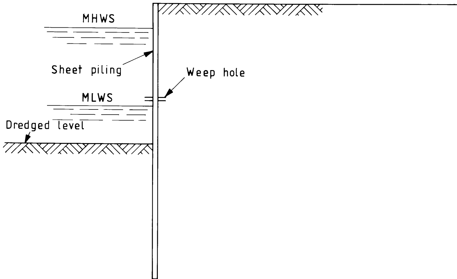
Figure 45 — Cantilevered single-wall sheet pile structure
