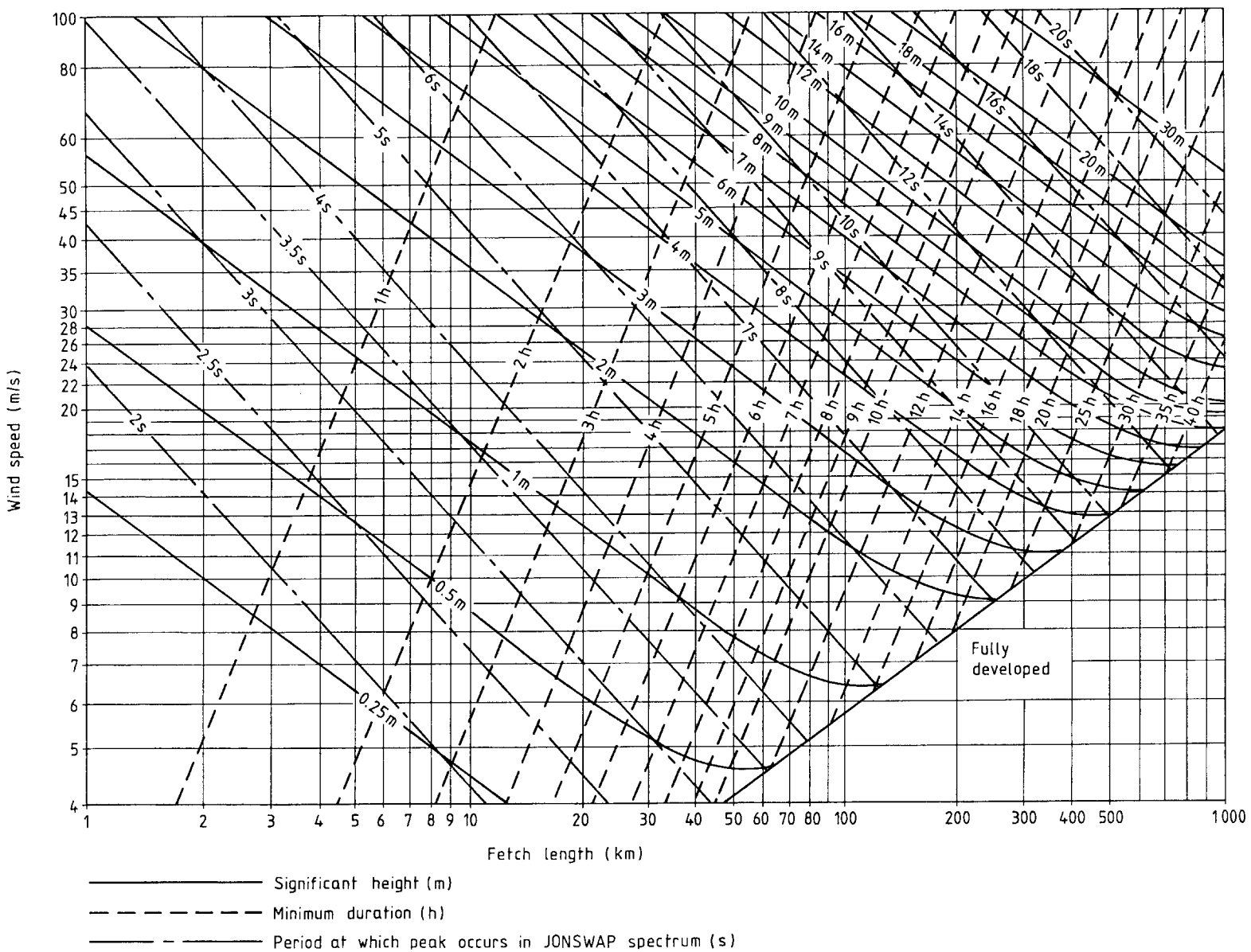
Figure 9 — Significant wave height and peak period for wave spectra
