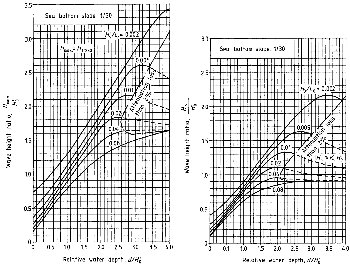
Figure 3e) — Wave shoaling and estimation of wave height in the surf zone (continued)
