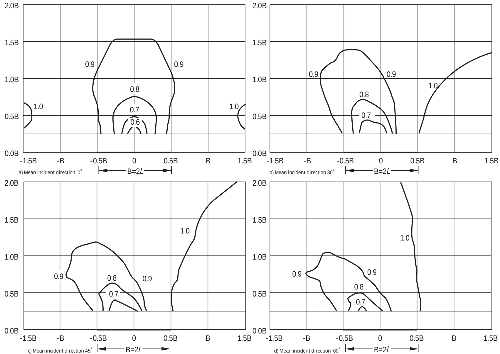
Figure 17b) Diffraction coefficients for island breakwater of length B = \text{two wave lengths} , Pierson-Moskowitz spectrum, \text{Cos}^2 directional spread. (Acknowledgement: HR Wallingford)
