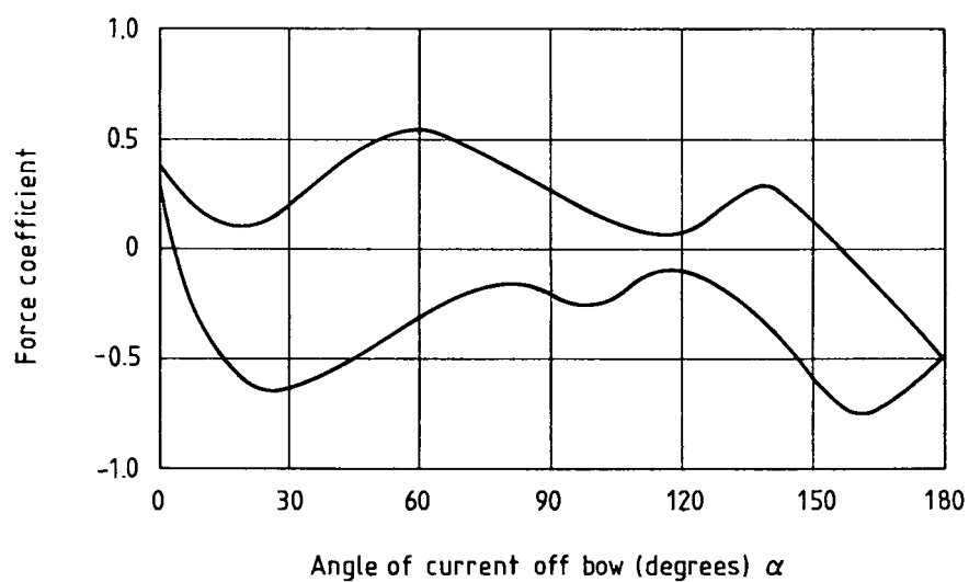
Figure 32 — Envelope of longitudinal force coefficients for VLCCs in shallow water
