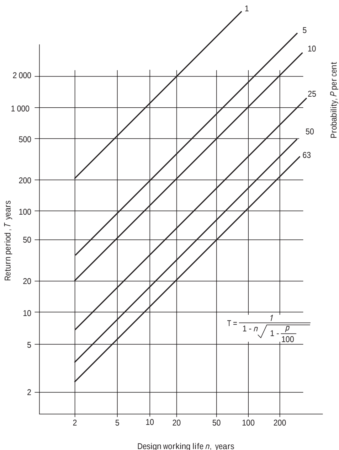
Figure 4 — Relationship between design working life, return period and probability of wave heights exceeding the normal average
