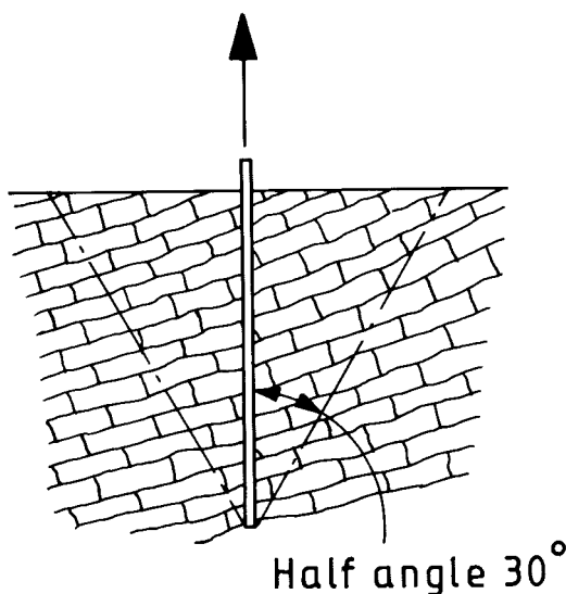
Figure 61 — Modes of failure of anchor tendons in rock — Thinly bedded rock with horizontal or near-horizontal bedding joints
