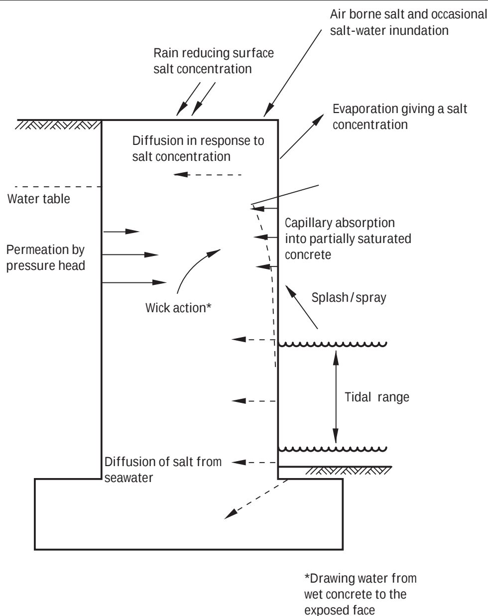
Figure 69 — Schematic diagram of the chloride transport processes in a maritime structure (Acknowledgement: The Concrete Society.)
