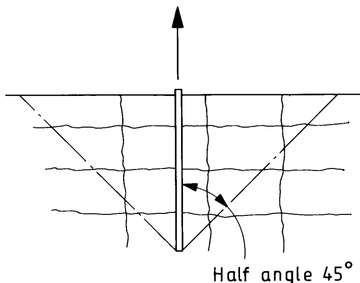
Figure 60 — Modes of failure of anchor tendons in rock — Massively bedded rock
