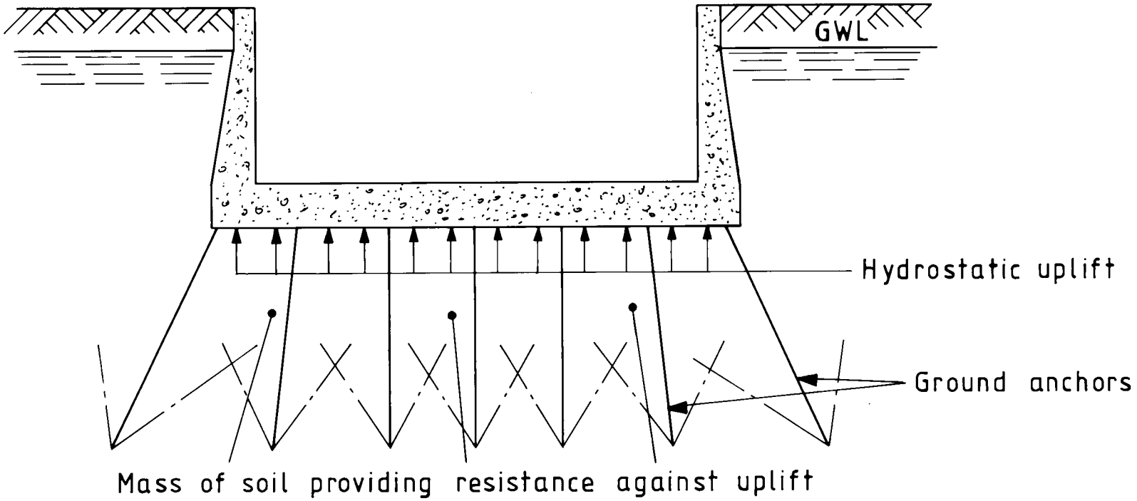
Figure 58 — Anchorage of lock or dry dock against hydrostatic uplift
