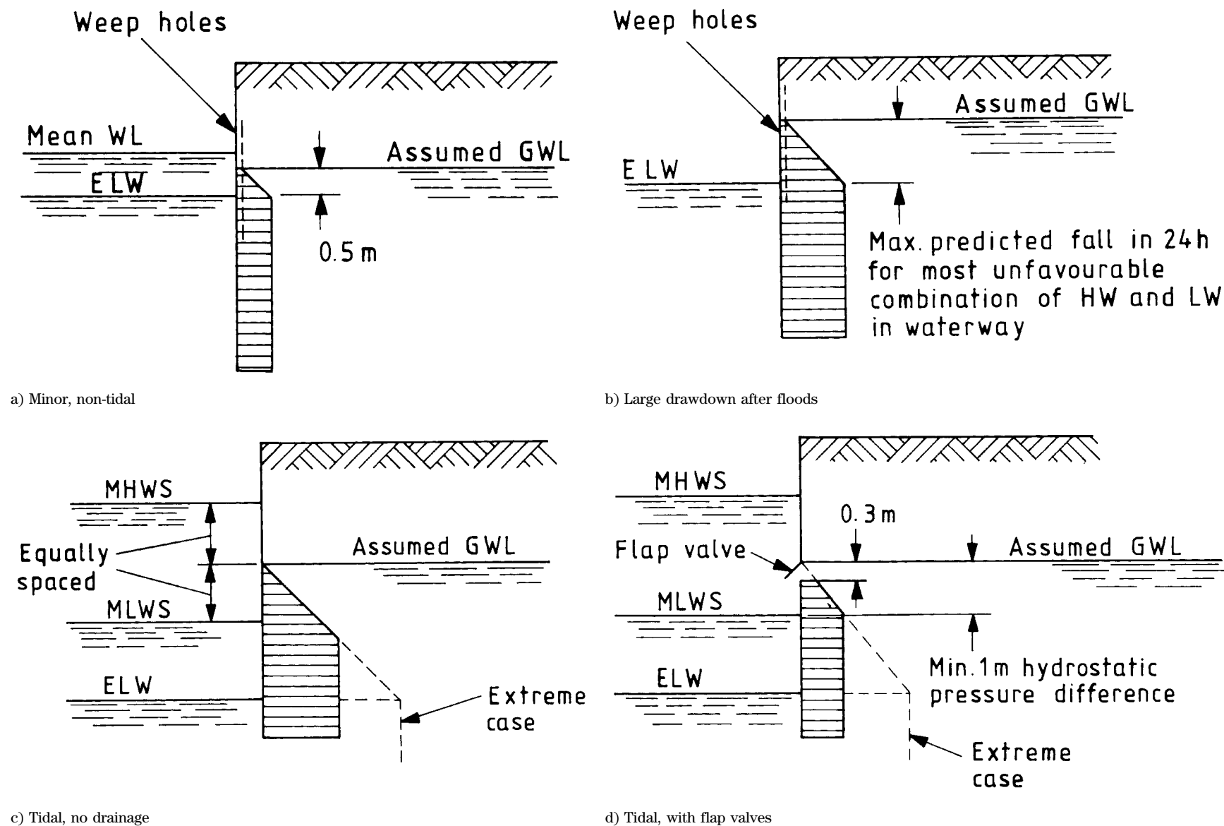
Figure 54 — Hydrostatic pressure distribution on waterfront structures where soil is retained to full height of structure
