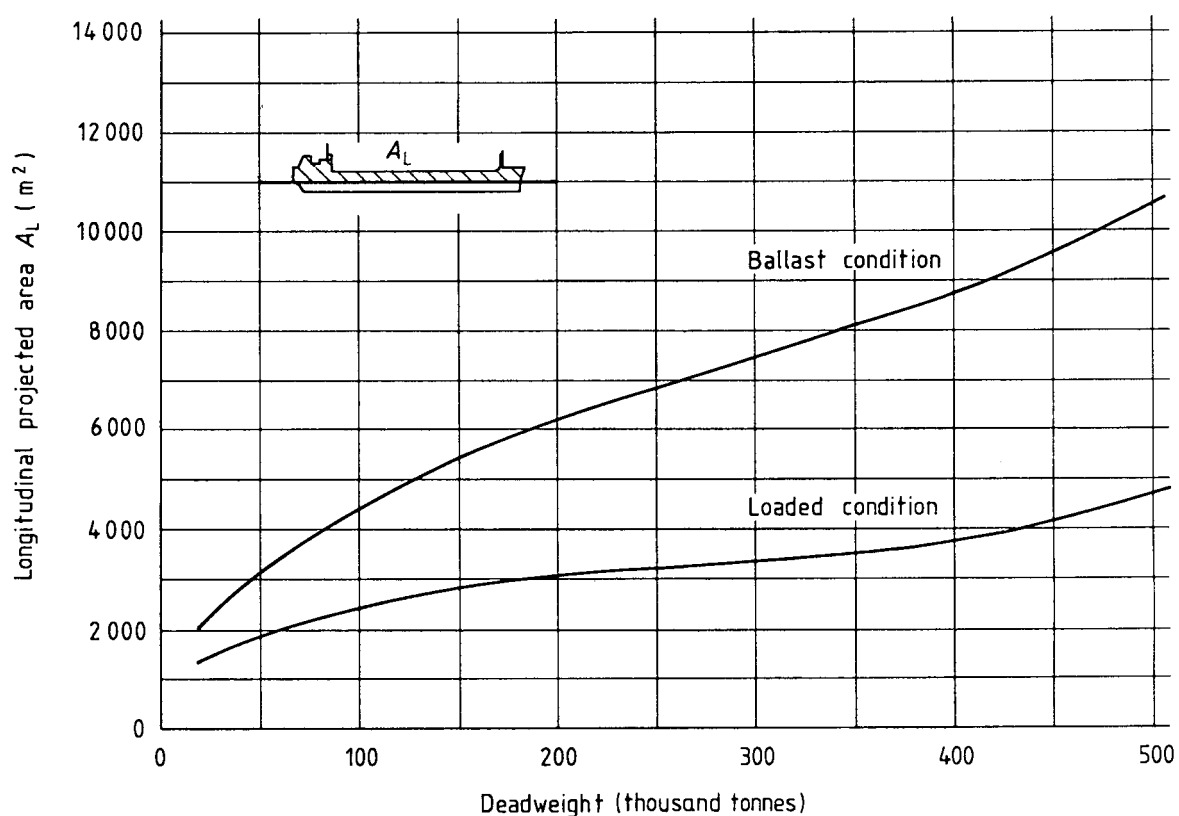
Figure 33 — Typical longitudinal projected areas of tankers
